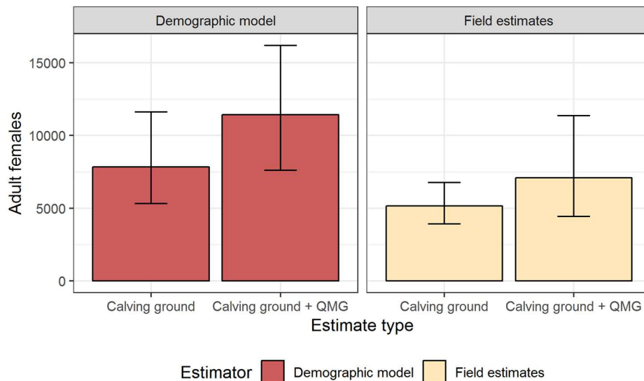
Figure 38: Field and model-based estimates of adult females on the Bathurst calving ground compared to estimates that were adjusted to include Bathurst females that calved on the Queen Maud Gulf coast calving area in 2018. Field estimates include the base estimate of adult females, and the base estimate of adult females divided by the proportion of collars that occurred on the Bathurst calving ground. Demographic model estimates include Bayesian IPM runs with the 2018 adult female estimate included and excluded.
