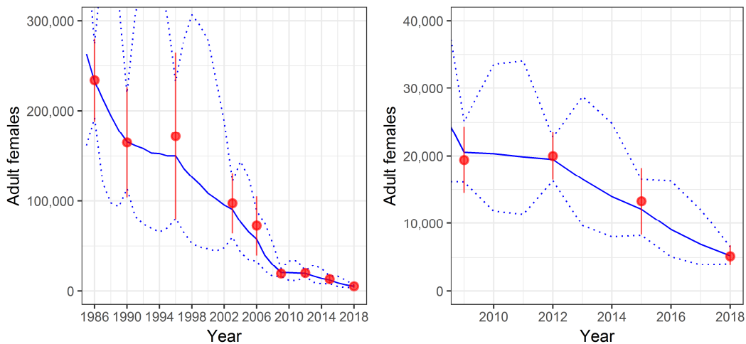
Figure 28: Trends in numbers of adult Bathurst females 1986-2018, as estimated by the Bayesian state space model. The left graph is for the full extent of the data set and the right graph is zoomed into the period of 2009-2018. Field estimates are given as red dots (with confidence limits) and model predictions are shown as blue lines with confidence intervals as hashed lines.
